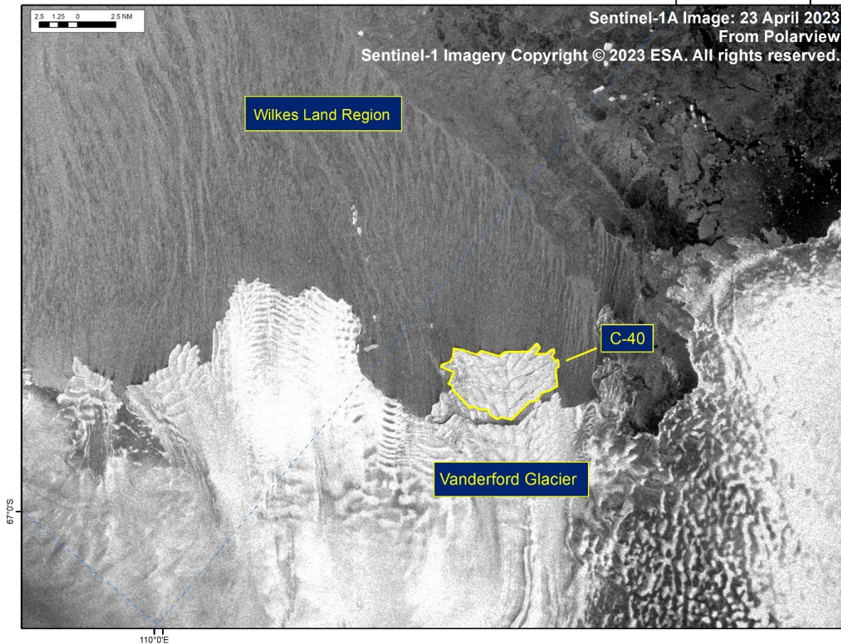
Figure 1: Sentinel-1A image of iceberg C-40 from April 23, 2023.
